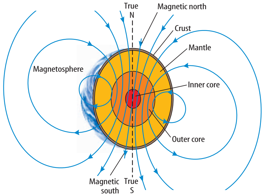
Figure 6 Earth has a magnetic field similar to the field of a bar magnet.
