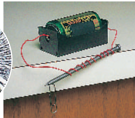
C An iron core inside the coils increases the magnetic field because the core becomes magnetized.
