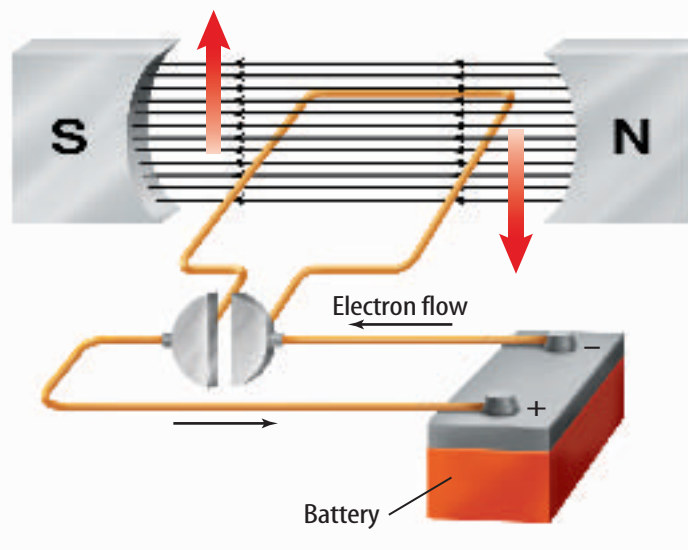
The magnetic field exerts a force on the wire loop, causing it to spin as long as current flows in the loop.
