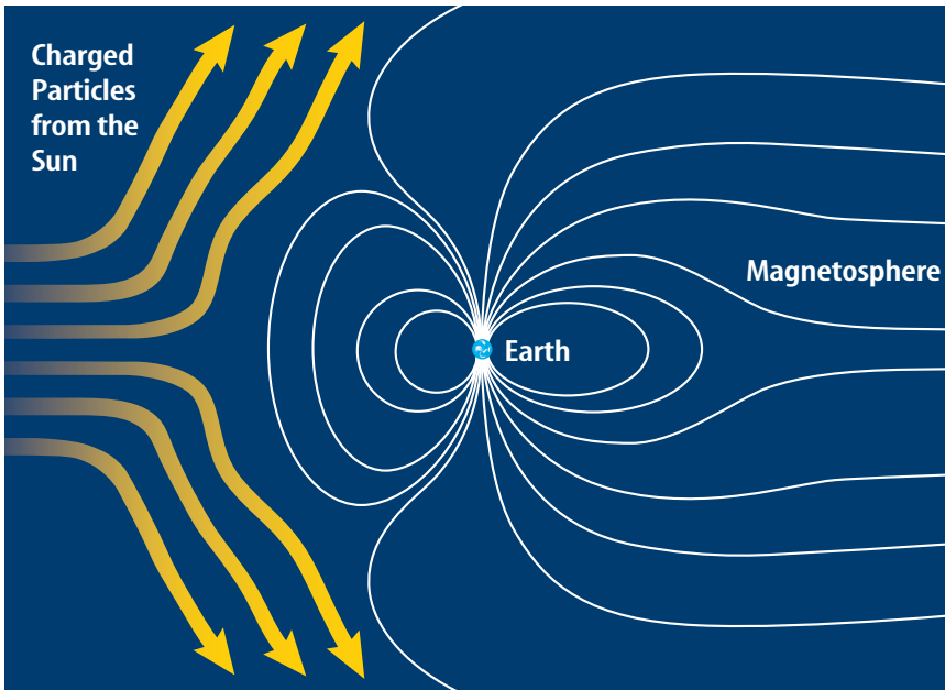
Figure 14 Earth's magnetosphere deflects most of the charged particles streaming from the Sun. Explain why the magnetosphere is stretched away from the Sun.
