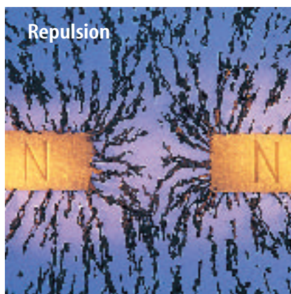
Figure 3 Magnetic field lines show attraction and repulsion. Explain what the field between two south poles would look like.
