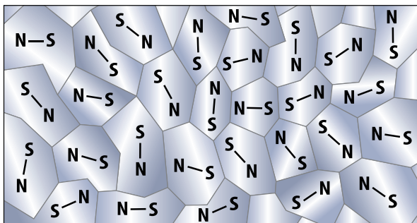
Figure 5 Some materials can become temporary magnets.
