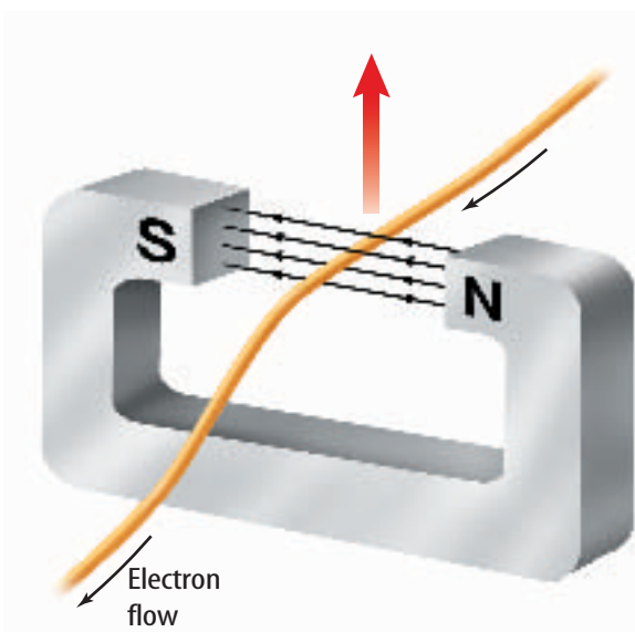
A magnetic field like the one shown will push a current-carrying wire upward.
