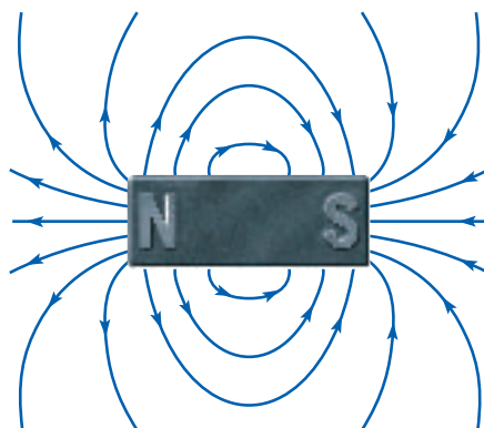
Figure 2 A magnetic field surrounds a magnet. Where the magnetic field lines are close together, the field is strong.
