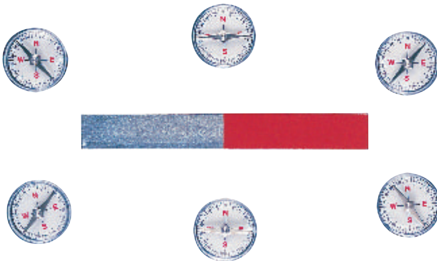
Figure 8 The compass needles align with the magnetic field lines around the magnet.
