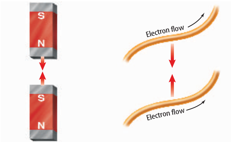
Figure 12 Two wires carrying current in the same direction attract each other, just as unlike magnetic poles do.
