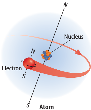
Figure 4 Movement of electrons produces magnetic fields. Describe what two types of motion are shown in the illustration.
